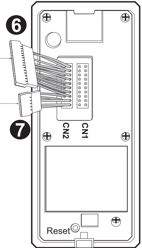
COSEC PATH RDFX/RDCX (Rear View)
